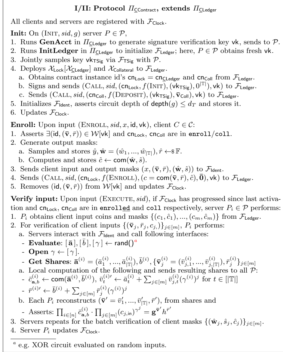
Fig. 12: Part 1 - Protocol \Pi_{\text{CContract}} UC-securely realizing \mathcal{F}_{\text{CContract}} .
