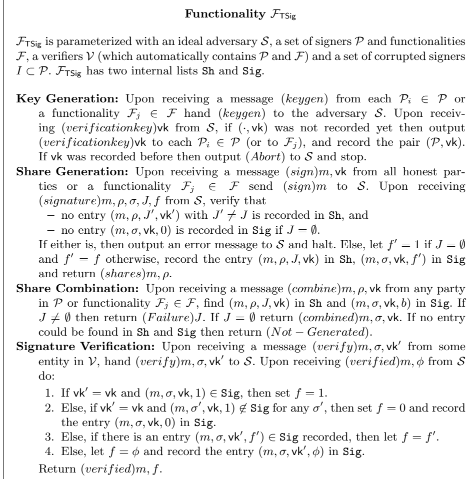
Fig. 4: Global UC functionality \mathcal{F}_{\text{TSig}} for Threshold Signatures.
